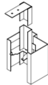
Plaster Partition Anchor (Ceiling Strut Optional)
